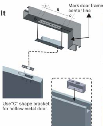
Standard Installation B1
